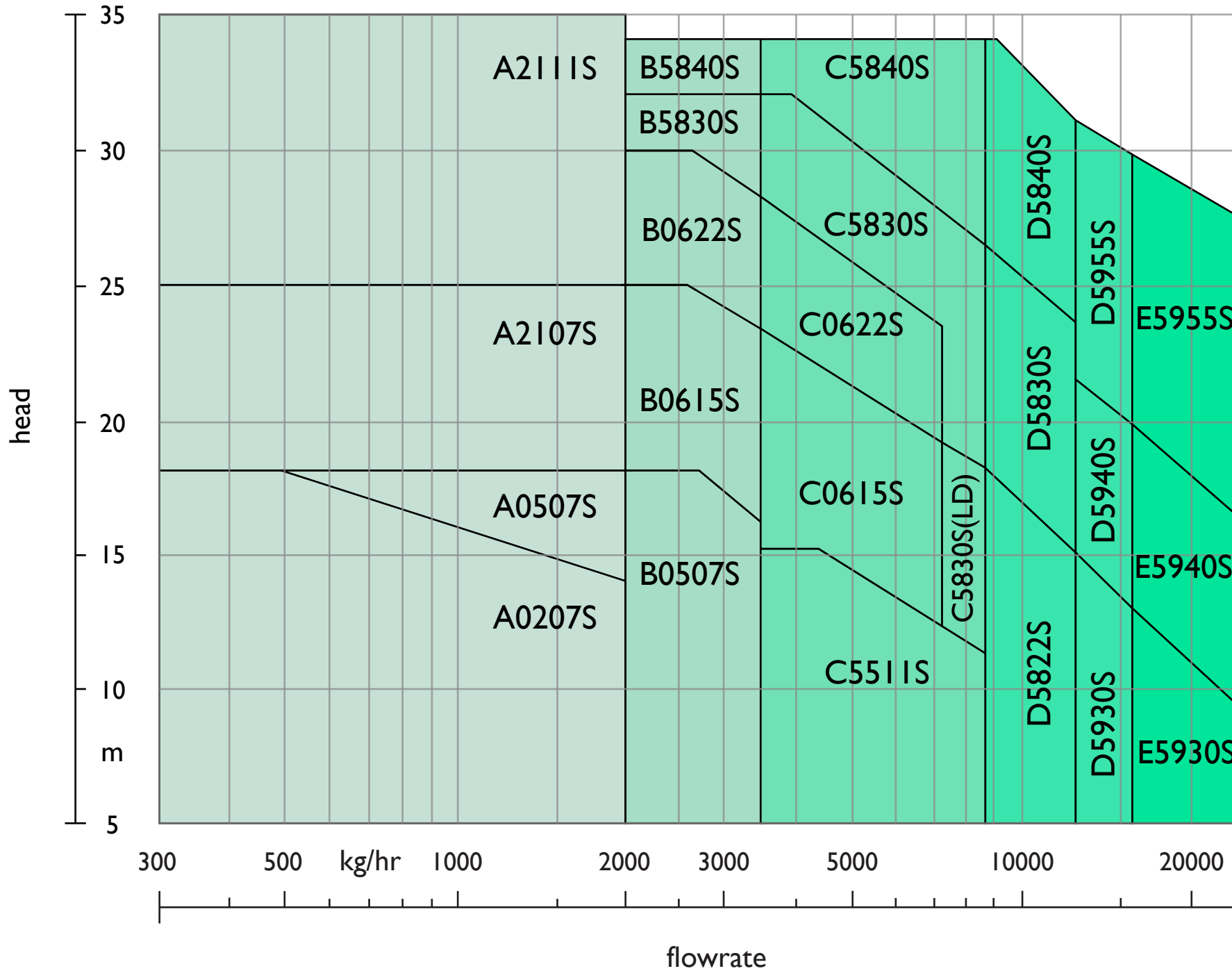
Series III single pump sizing chart at 94 °C
