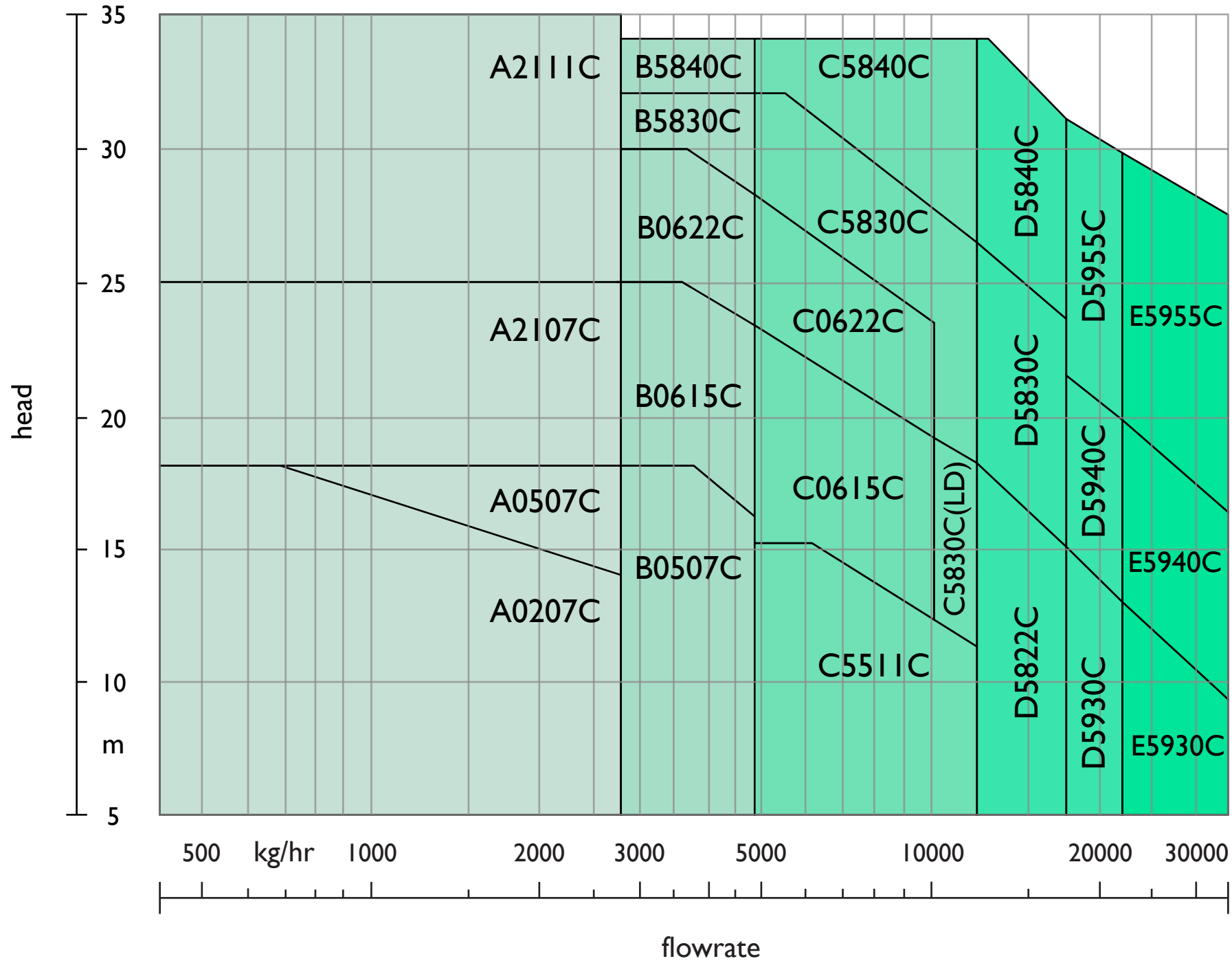
Series III duplicate pump sizing chart at 94 °C
