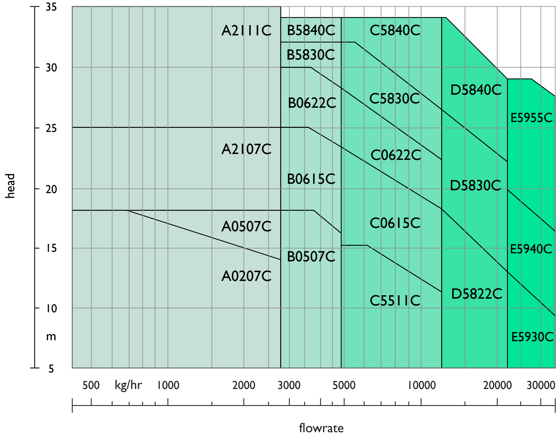
Series III duplicate pump sizing chart at 90 °C
