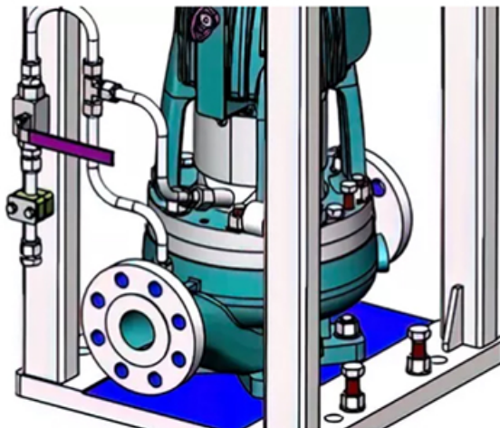
Computer model of the Amarith API 610 Vertical In-line Pump designed for the Yanbu refinery, Saudi Arabia - Image courtesy of Amarith.
