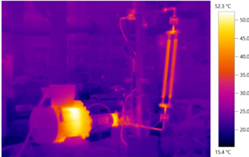
A thermal image of an Amarith pump in operation undergoing IECEX certification. (Image source: Amarith Ltd.)
