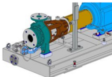
3D CAD model of an Amarith titanium pump being designed for WWS Westgarth to be installed aboard an FPSO vessel.
