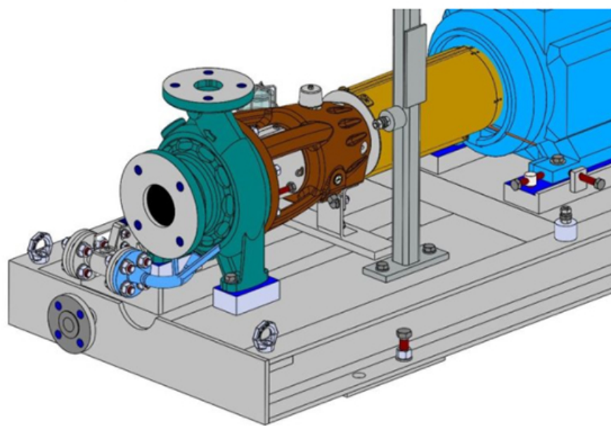
3D CAD model of an Amarith titanium pump being designed for VWS Westgarth to be installed aboard an FPSO vessel. (Image source: Amarith)
