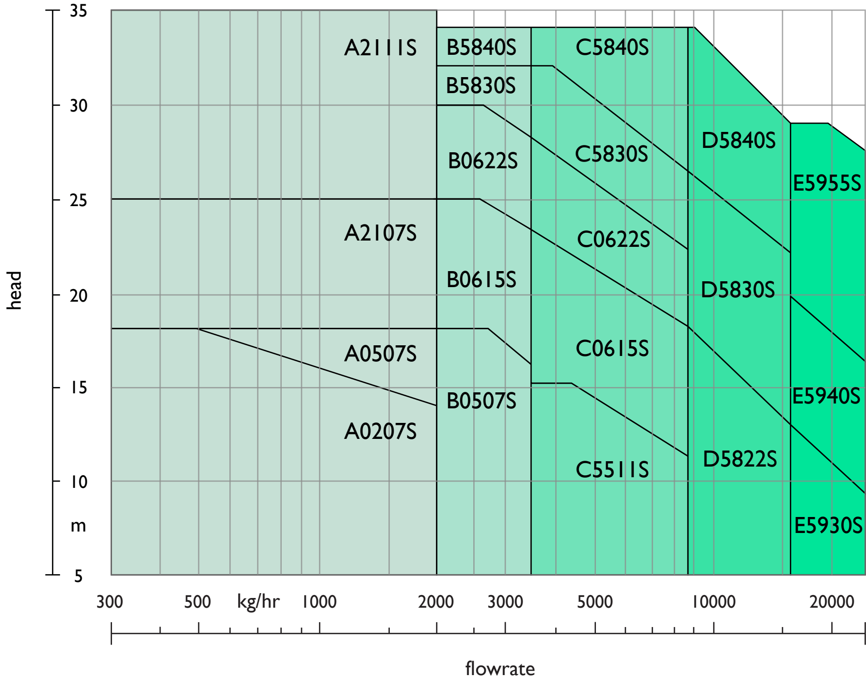
Series III single pump sizing chart at 90 °C
